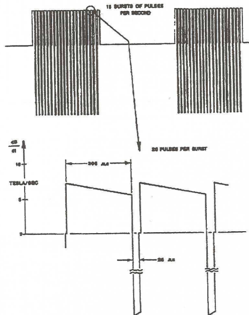
Figure 6 The original signal for treatment of non-union fractures proposed by Bassett et al.
